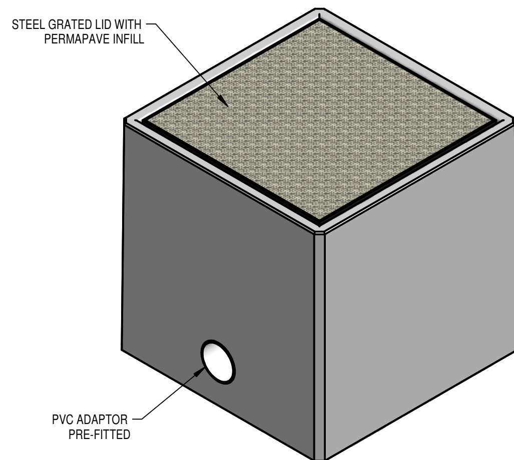
SENTINEL PIT AS SUPPLIED (N.T.S)
