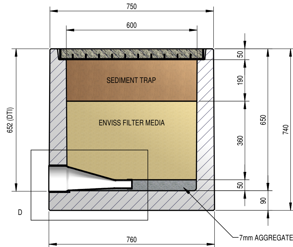
600x600x650 RKO PIT (1:10)
