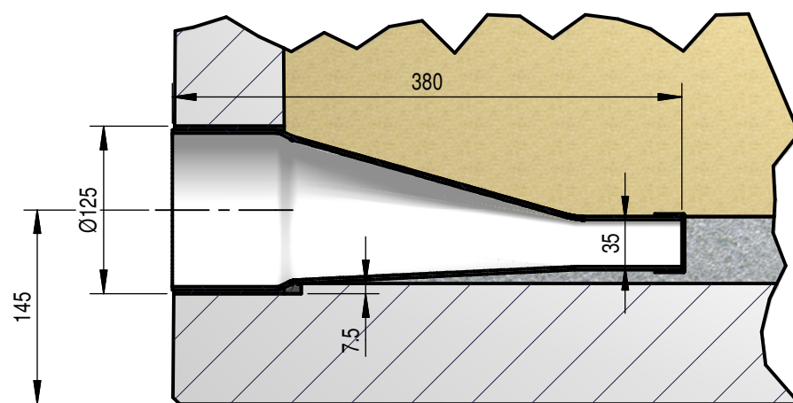
DETAIL D (1:5)
